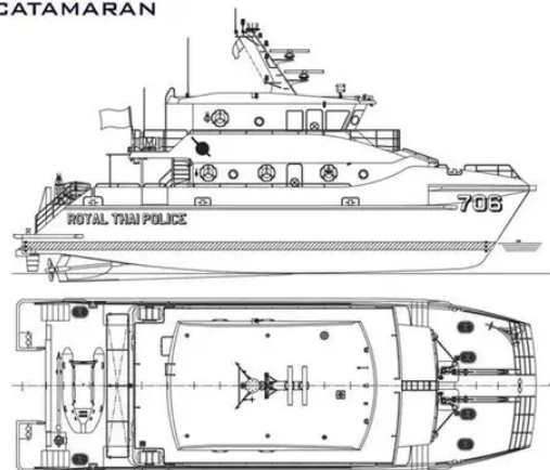
23М. CATAMARAN
